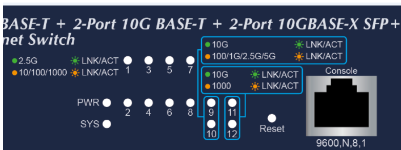
Figure MGS-6311-10T2X front panel
