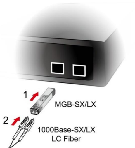
Figure 2-16 Plug in the SFP transceiver
