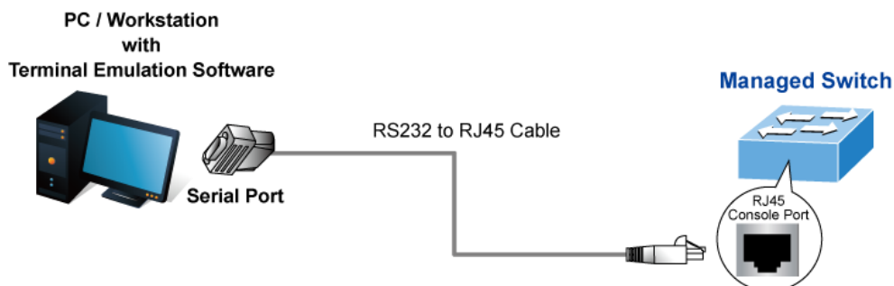
Figure 4-1 Managed Switch Console Connectivity
