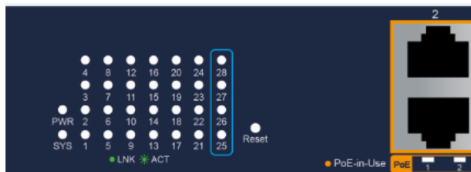
Figure GS-6311-24P4XV front panel
