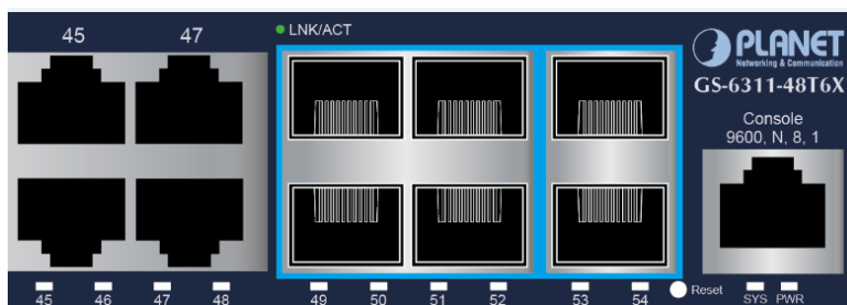
Figure GS-6311-48T6X front panel
